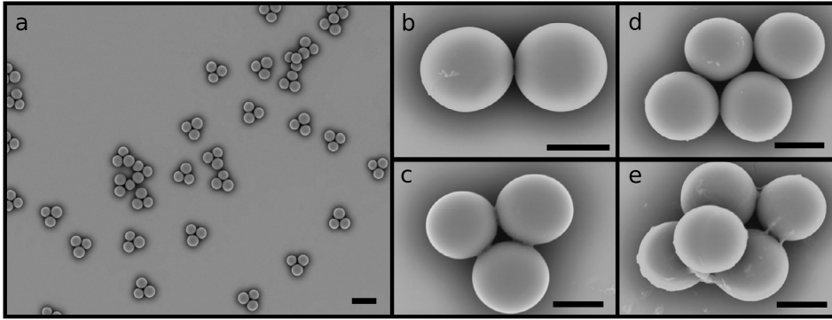
Fig. 1. Self-assembled colloidal clusters. a) Electron micrograph of a suspension of triplet clusters. Scale bar, 30 \mu\text{m} . b–e) Close up of doublet, triplet, quadruplet, and quintuplet clusters. Scale bars, 10 \mu\text{m} . Further details are available in [7], photograph courtesy of Dr. Joshua Ricouvier.
