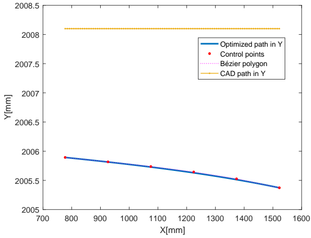
Figure 7: Tool path in robot world y direction
