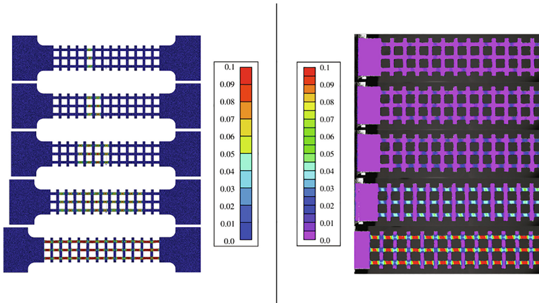
Fig. 29. e_1 strain map in the tensile direction for the 0^\circ -oriented square lattice with comparison of the simulation on the left to the experiment on the right.
