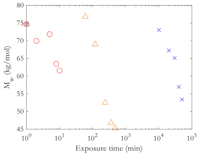
Fig. 7. Average weight molar mass changes for thermal ageing at 210 °C (○), 180 °C (△) and hydrolytic ageing at 80 °C (×). Values are given in PMMA equivalent.
