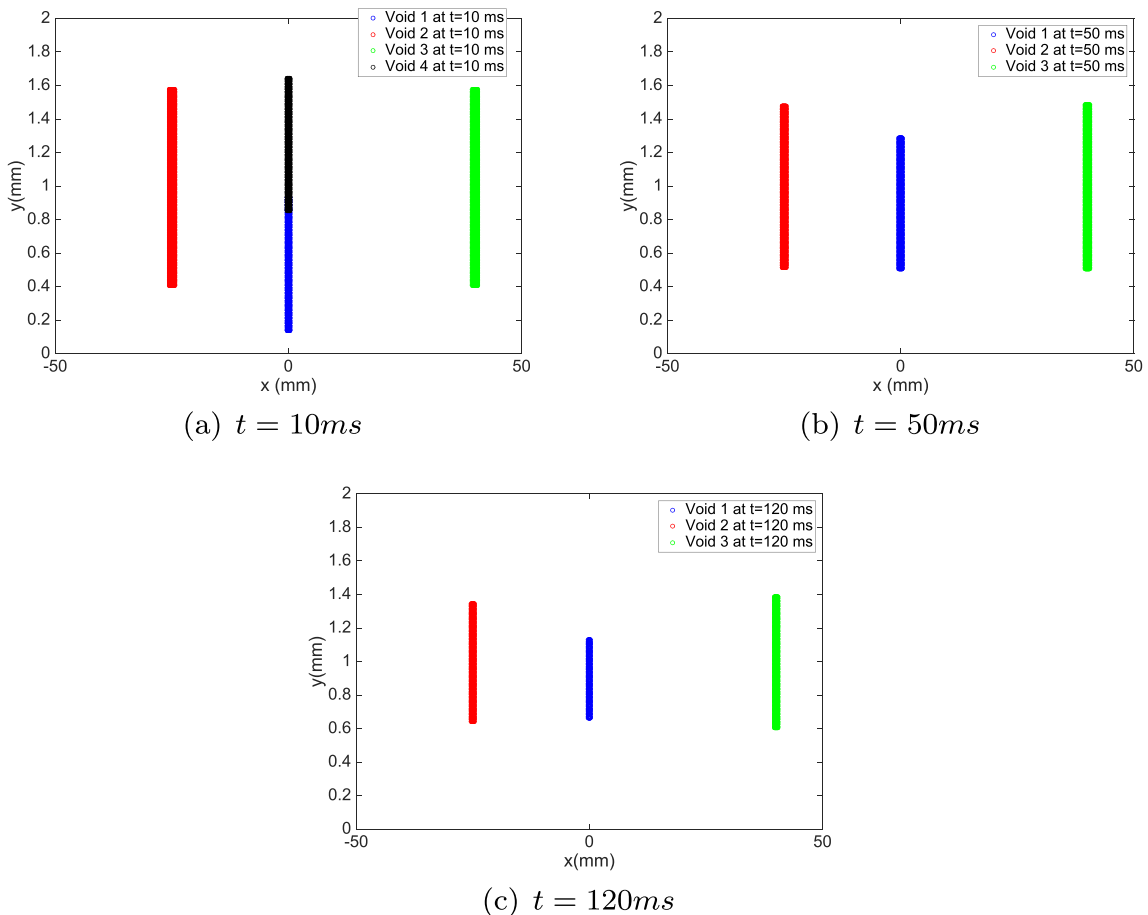
Fig. 13 Merging two overlapping voids, compression at u = 0.1mm/s
