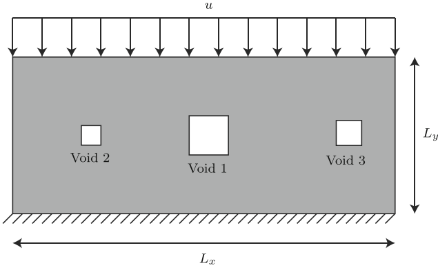
Fig. 4 The considered simple domain (in which L_x and L_y are the width and the thickness of the tape respectively) containing three voids of different sizes. Initially Void 1 is 1.5 \times 1.5mm^2 , voids 2 is 1 \times 1mm^2 and void 3 is 1.25 \times 1.25mm^2 in the first example illustrated in Section 3
