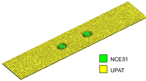
Figure 7: meshing of the sample plate
