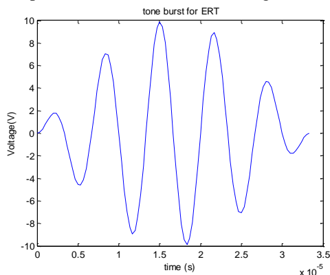
Figure 8: Tone burst, A=1V , f_0=100kHz , N_c=5
