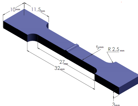
Fig.6: Specimen tensile test dimensions
