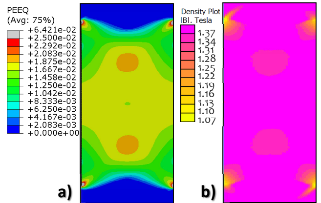
Fig.17: The finite element model simulating the local deformed sample, a) the equivalent plastic strain, b) the magnetic flux distribution (sample S_{hr1} ).
