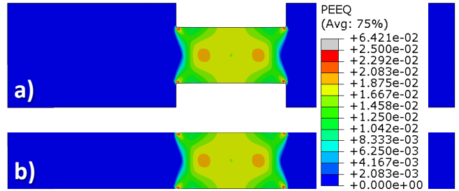
Fig.16: The mechanical finite element simulation of a local deformation (sample S_{hr1} ).
