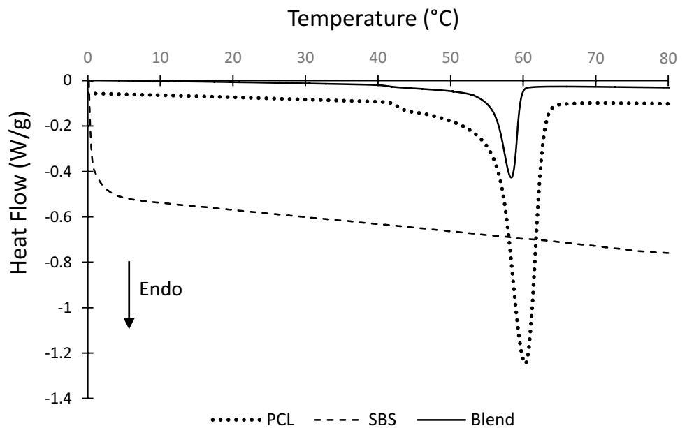
Fig. 2 Results of DSC tests on pure PCL a , pure SBS b and the blend.
