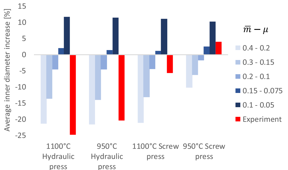
Fig. 9 Influence of friction coefficients on the samples' inner diameter variation after the ring compressions tests
