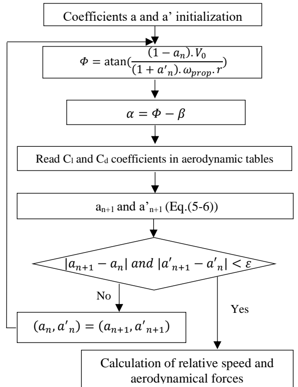
Figure 3: Fixed-point algorithm
