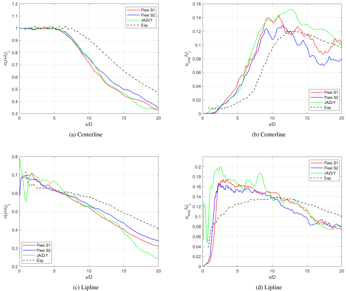
Figure 2: Results of mean longitudinal velocity component distribution (left) and rms of longitudinal velocity fluctuation (right) in the jet centerline y/D = 0 (top) and lipline y/D = 0.5 (bottom).
