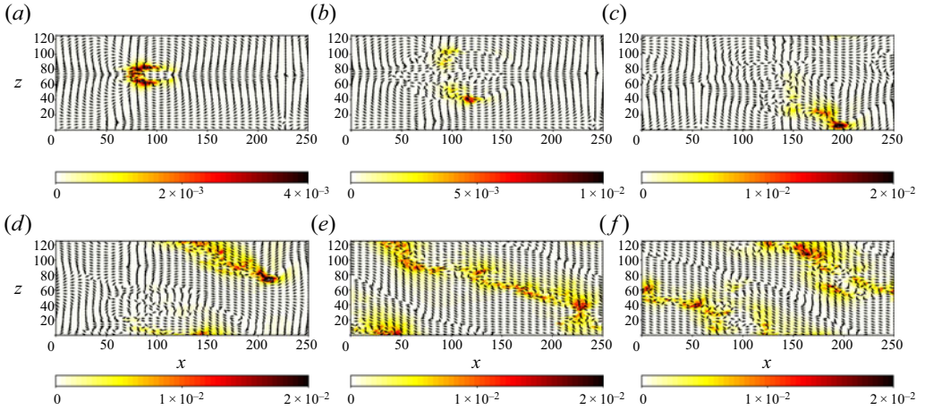
Figure 15. Isocontours of the crossflow energy E_{cf} together with the normalized y -integrated large-scale flow (vectors) for several instantaneous fields ( Re = 1000 , E_0 = 5.5 \times 10^{-7} , T = 100 ): (a) t = 150 , (b) t = 500 , (c) t = 900 , (d) t = 1500 , (e) t = 2500 , (f) t = 3000 .
