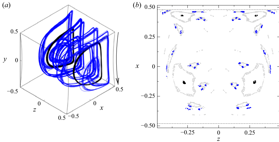
Figure 23. Nine trajectories for a = 0.0069 ( a_p = 0.28 mm) and \varrho = 1.022 recorded during t \in [3000, 3600] s. (a) Three-dimensional view of the period-one (black) and period-twelve (blue) attractors. (b) Poincaré sections on the plane y = 0 (black, blue) of the particle trajectories shown in (a). Poincaré sections of numerically computed streamlines on the corresponding largest reconstructible KAM tori are shown as light grey dots.
