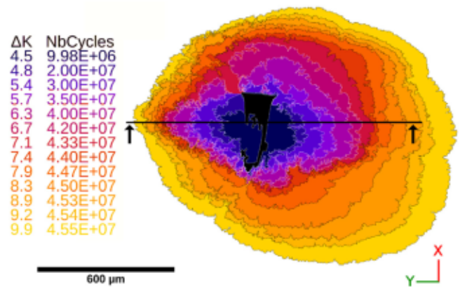
Fig. 8. Crack shape projections at different propagation stages on a plane perpendicular to the loading direction. The stress amplitude is 330 MPa with a vacuum environment (specimen n° 46). The cutting plane indicated by arrows corresponds to the section depicted in Fig. 7. The displayed Stress Intensity Factor range \Delta K is calculated as detailed in Section, 4.3.
