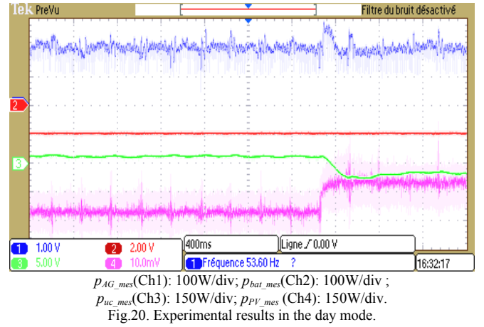
Fig. 20. Experimental results in the day mode.
