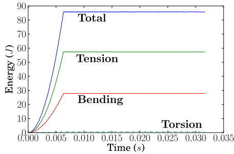
Figure 12: Energy breakdown of total elastic energy stored by cohesive beams for the quasi-static tensile test (computed with a time step \Delta t = 3.10^{-7}s and a number of iteration it = 100\,000 )
