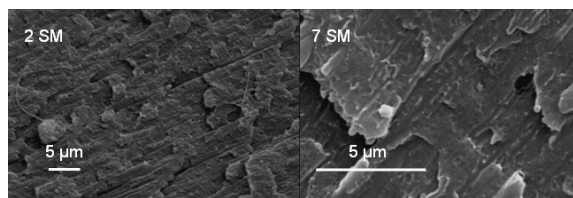
Figure 4: SEM micrographs of ABS/PA/SMA3000 (70/30/5) obtained with CM method (2 and 7 SM)
