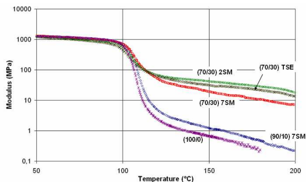
Figure 3: DMTA curves of ABS and ABS/PA blends obtained with the two methods, TSE and CM (2 and 7 SM).
