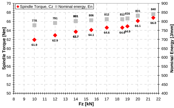
Figure 4: Spindle torque C_z and Nominal energy E_n evolution as the axial force process range
