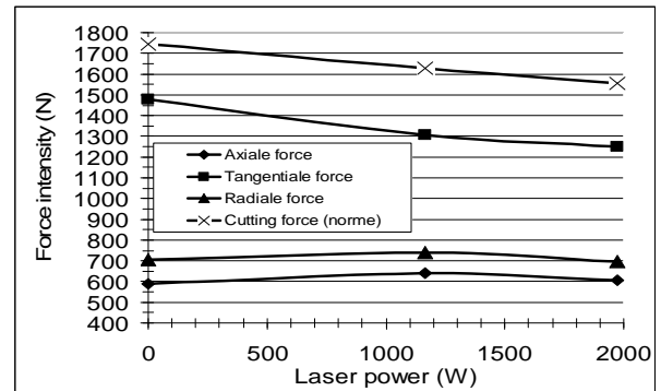
Fig 3: Evolution of the three components and the magnitude of the cutting force as a function of the laser power
