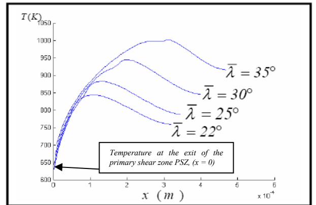
Figure 3 : Effect of the global friction coefficient \bar{\mu} = \tan(\bar{\lambda}) on the temperature distribution at the tool chip interface.
