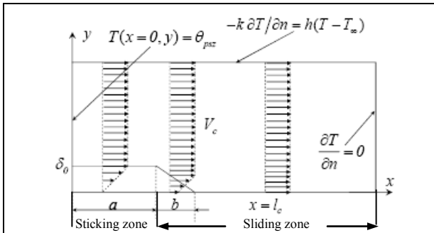
Figure 2 : Illustrations of the velocity distribution in the chip and of the thermal boundary conditions
