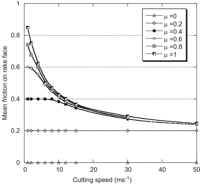
Fig. 3. Effect of the cutting speed V on the mean friction coefficient \bar{\mu} (accounting for the contact forces exerted on the tool rake face II , see Fig. 1b). Various values of the sliding friction coefficient \mu are considered. Note that \bar{\mu} = \mu for small values of \mu since sticking does not occur in that case. For large values of \mu , it appears that \bar{\mu} < \mu and that \bar{\mu} is a decreasing function of V as a result of thermal softening of the work-material along the secondary shear zone. For \mu=0.4 and 0.6 it is observed that \bar{\mu} is tending to \mu for small values of the cutting speed, as sliding contact is dominant.
