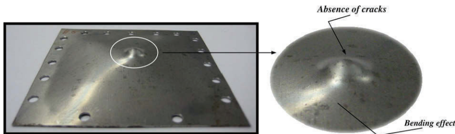
Fig. 30. Petalling failure mode for V_0 = 2.9 m/s and T_0 = 213 K. Dry condition.
