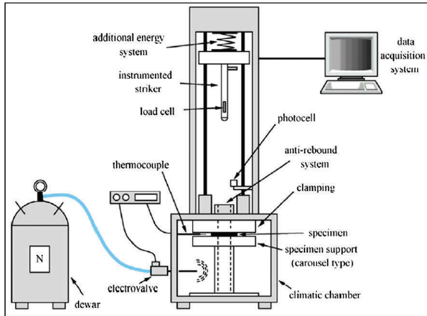
Fig. 9. Schematic representation of the drop weight tower.
