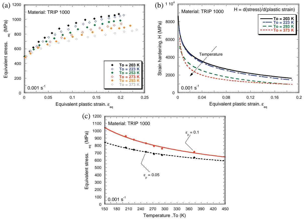
Fig. 7. (a) Flow stress of TRIP 1000 as a function of plastic strain for different initial temperatures. (b) Strain hardening of TRIP 1000 as a function of plastic strain for different initial temperatures. (c) Evolution of the flow stress as a function of temperature for different plastic strain values.
