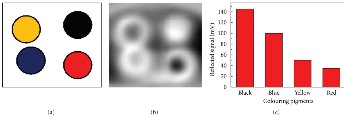
FIGURE 4: (a) Sample design (50 mm × 50 mm), (b) reflection image at 110 GHz, white colour indicating higher reflection, (c) corresponding curve revealing the difference in reflection by various colour pigments.
