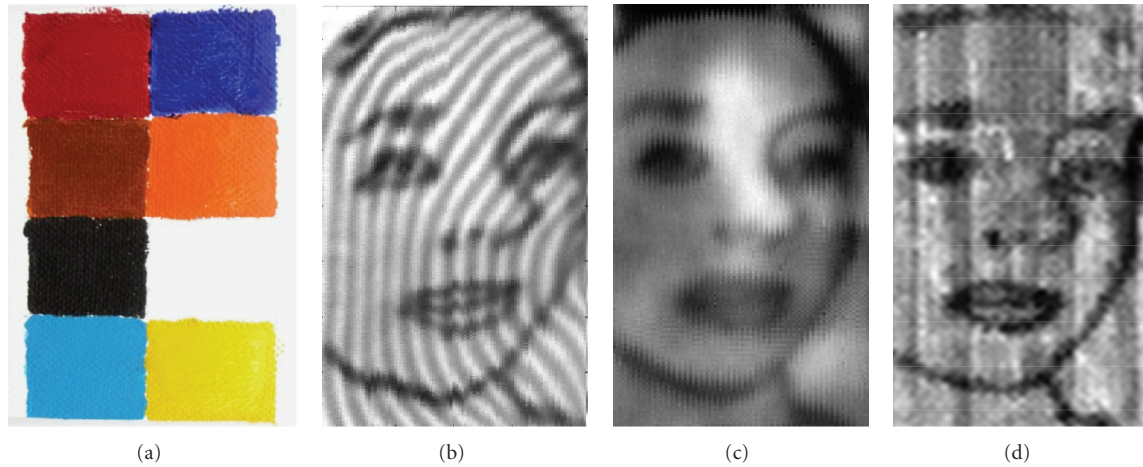
FIGURE 2: (a) Photograph of the sample (paint layers covering a graphite sketch), (90 mm × 55 mm); (b) transmission CW image at 240 GHz; (c) transmission CW image after application of a FFT bandpass filter (Image J software) to remove background interference pattern; (d) transmission pulsed THz image at 240 GHz. In (b) to (d), black level indicates a decrease of THz signal.
