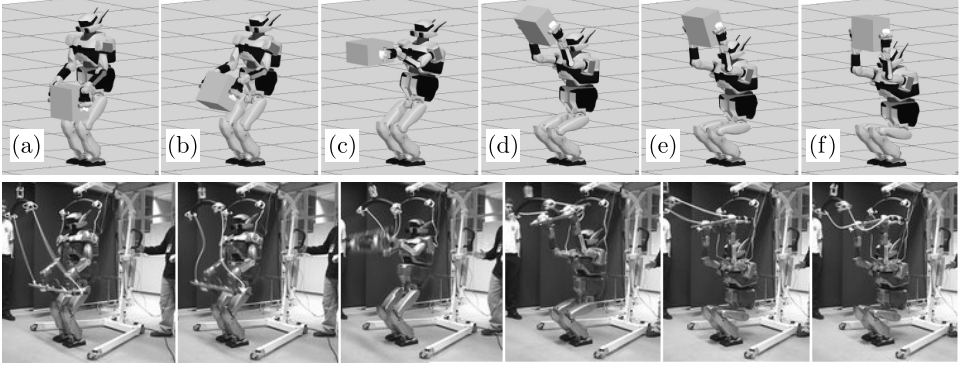
Fig. 14. HRP-2 robot lifting a 8.4kg object using an optimized trajectory generation software (up: simulation. Down: experiment). From left to right: (a) initial state, (b) accelerating the object upward, (c) switching motion, (d) sliding into under the object, (e) crouching, (f) final state (sitting). The robot also succeeded in lifting a 23.4 kg object.
