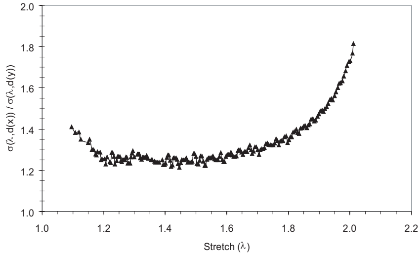
Fig. 5. For the 50 phr carbon-black filled SBR, ratio of the stress unloading response of the material stretched to 100 % (x=2) over the stress unloading response of the material stretched to 200% (y=3), vs. stretch \lambda .
