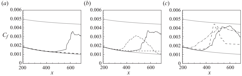
FIGURE 17. Distribution of the mean skin friction coefficient C_f at t=700 for the base flow initially perturbed by: the global three-dimensional optimal (—); the local optimal with \alpha=0 (---); the suboptimal with \alpha=\beta_{opt} (- · - · -). Three initial energy levels are considered: E_0=0.5 (a); E_0=2 (b); and E_0=10 (c). The lowest and highest thin lines represent the theoretical distributions of the mean skin friction coefficient for a laminar and a turbulent boundary layer, respectively.
