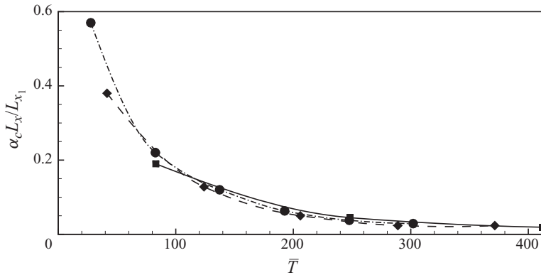
FIGURE 6. Normalized most amplified longitudinal wavenumber versus the normalized target time at Re = 610 , for L_{x1} = 400 (■), L_{x2} = 800 (◆) and L_{x3} = 1200 (●).
