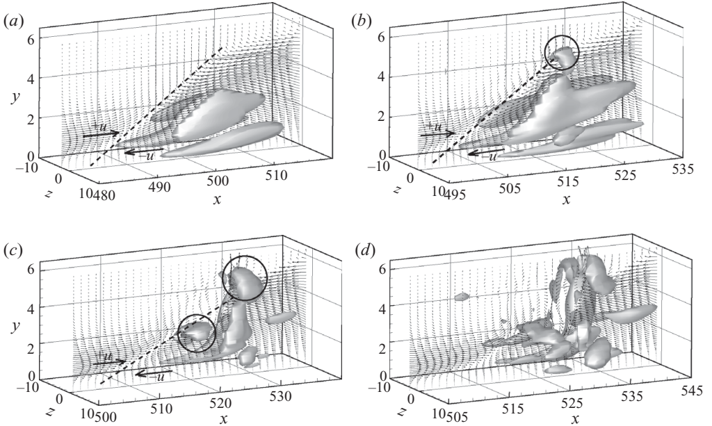
FIGURE 22. Iso-surfaces of the Q parameter and perturbation velocity vectors on the z=0 plane at t = 145 (a), t = 165 (b), t = 180 (c) and t = 190 (d). The surfaces represent the positive values Q = 370 for (a) and (b) and Q = 700 for (c) and (d). The inclined shear layer is represented by the dashed line in (a–c).
