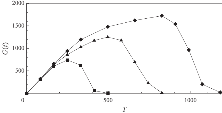
FIGURE 4. Envelope of the optimal energy gain computed by the direct-adjoint method at Re = 610 for three longitudinal domain lengths, L_{x1} = 400 (■), L_{x2} = 800 (▲), L_{x3} = 1200 (◆).
