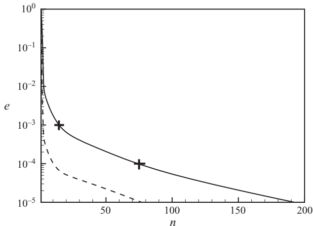
FIGURE 13. Normalized increment of the objective function versus the number of direct-adjoint iterations represented in a semilogarithmic scale for a computation initialized using a wave packet (—) and a single-wavenumber perturbation (---) for T=247 and \beta_L=0.1 . The crosses indicate the convergence levels at which the ‘near-optimal’ wave packets have been extracted.
