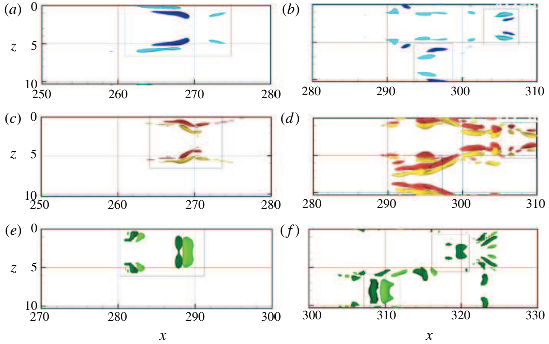
FIGURE 21. (Colour online) Isosurfaces of the lift-up term v'U_y = \pm 0.04 at t = 75 and t = 125 ( a and b , respectively); of the term (w'w')_z = \pm 0.025 at t = 75 and t = 125 ( c and d , respectively); of the Uv'_x = \pm 0.13 term at t = 100 and t = 150 ( e and f , respectively).
