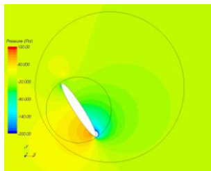
Fig. 20. contours de pression, \theta=216 degrees, a15i
