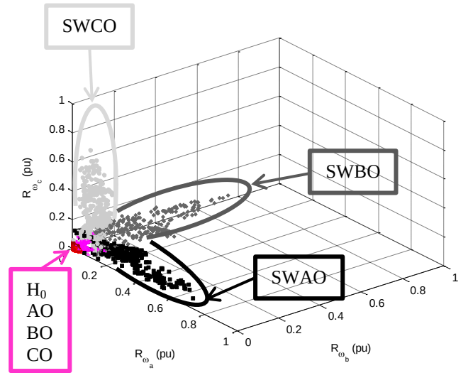
Fig. 13. Frequency-based fault indices for the six faults under study.
