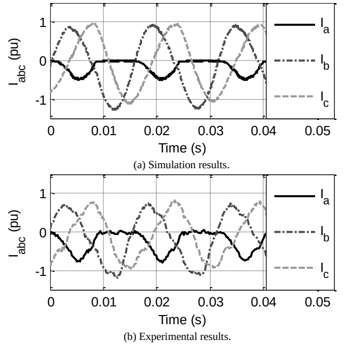
Fig. 4. Comparison of the phase currents obtained by simulations and by experiments with an open-switch fault (SWA1O) with \omega_m = 100\text{ rad s}^{-1} and I_a^* = 0.7\text{pu} .
