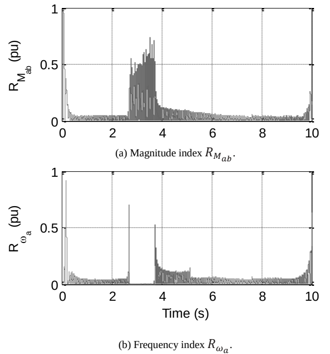
Fig. 17. Fault indices obtained under non-stationary and healthy conditions.
