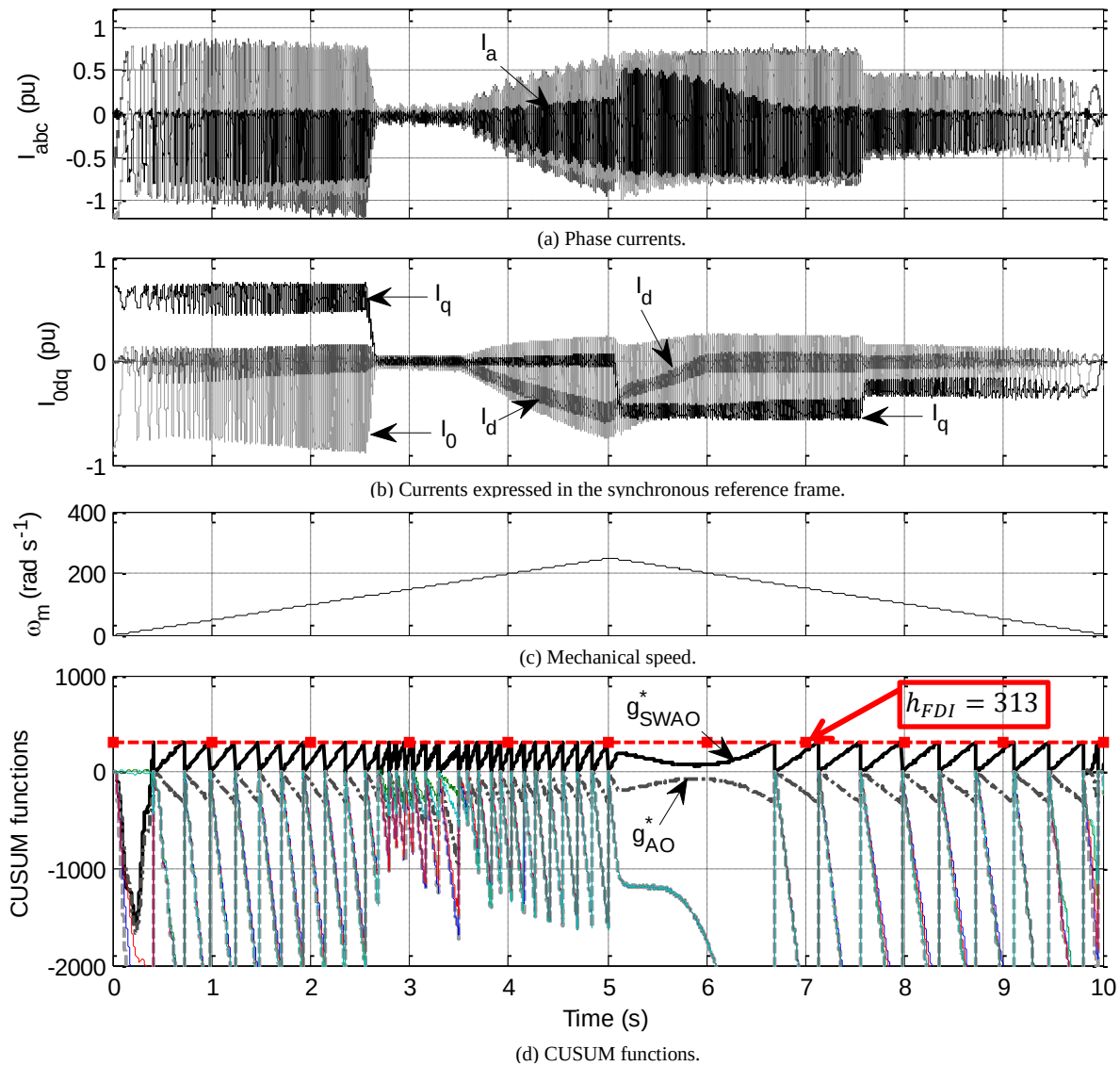
Fig. 18. Experimental results of the proposed FDI scheme under non-stationary conditions with a single-switch open-circuit fault (SWA10).
