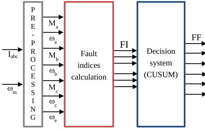
Fig. 1. Block diagram of the FDI scheme.
