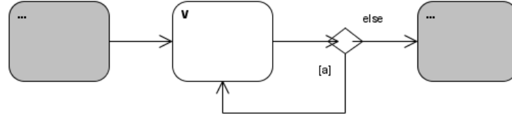
Fig. 15. Until pattern in UML
