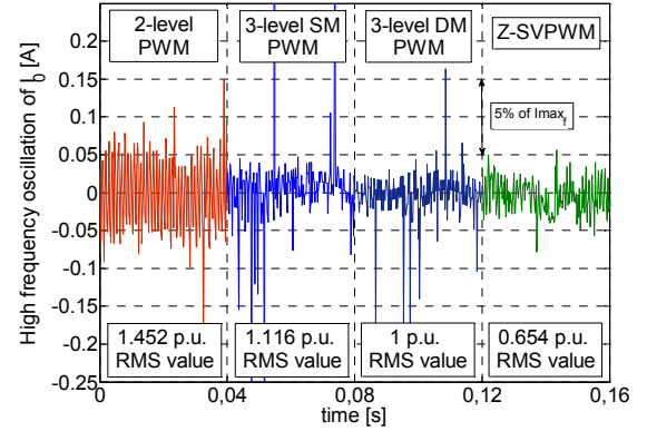
Fig. 10. Experimental results on the zero sequence current
