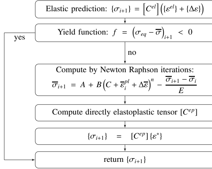
Figure 5: Incremental deformation algorithm
