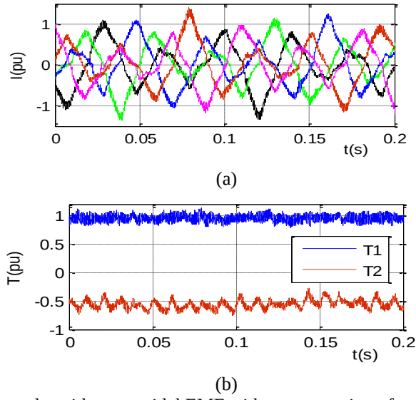
Fig.11. Experimental results with trapezoidal EMF with compensation of torque ripples and the two machines at different constant speeds: (a) Current in five phases of inverter, (b) torque.
