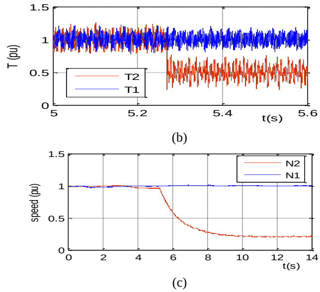
Fig.12. Experimental result with trapezoidal EMF in transient operation: (a) Current in the five phases of inverter, (b) torques and (c) speed of the two machines.
