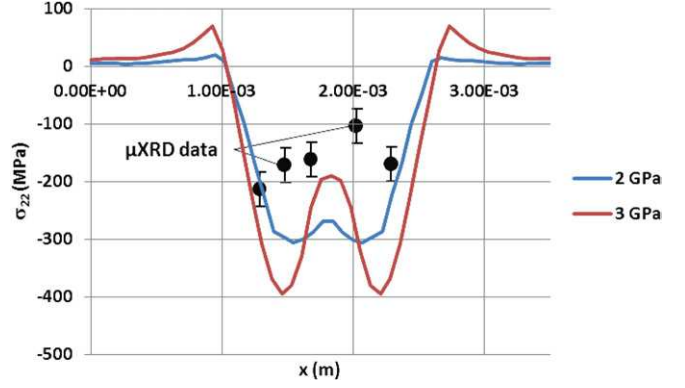
Figure 14. Residual stresses induced by a single laser impact at I_0 = 3.5 \text{ GW cm}^{-2} (2050-T8)—experiments versus simulation at impact pressures P_0 = 2 and 3 \text{ GPa} .
