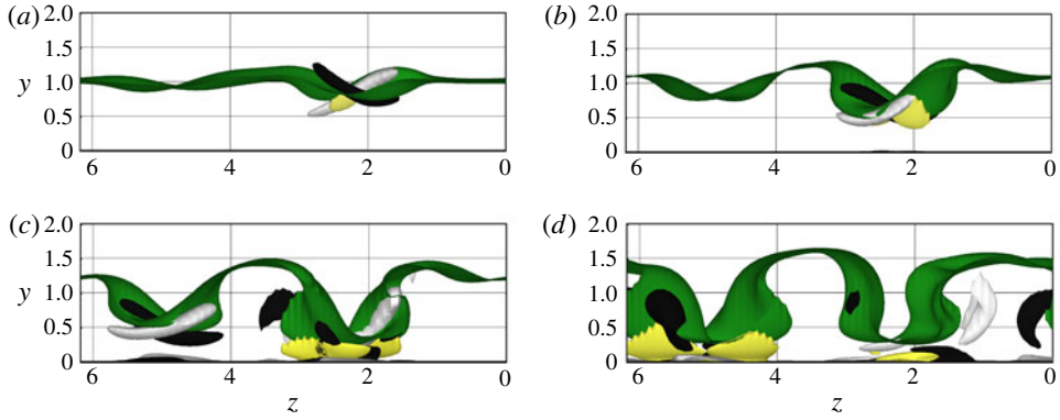
FIGURE 21. (Colour online) Null streamwise velocity contours (dark, green online), streamwise vorticity perturbation (black and pale grey for positive and negative values), and local dissipation rate (light, yellow online), extracted from a DNS initialized by the nonlinear optimal disturbance obtained for E_0 = 0.01 and T = 50 , at times (a) t = 10 (surfaces for \omega_x = \pm 0.6 , \epsilon = 5 ), (b) t = 30 (surfaces for \omega_x = \pm 0.6 , \epsilon = 12 ), (c) t = 50 and (d) t = 70 (surfaces for \omega_x = \pm 0.6 , \epsilon = 16 ).
