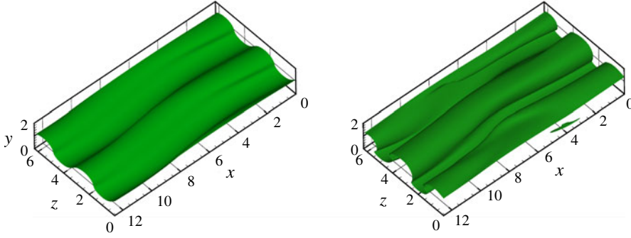
FIGURE 19. (Colour online) Null streamwise velocity contours for (a) the equilibrium solution found by bisection, and (b) a snapshot extracted at t = 80 by the DNS initialized by the short-path perturbation.
