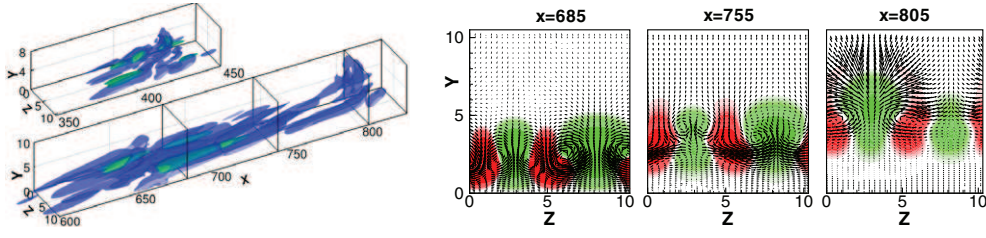
Figure 5. Snapshots of the streamwise component of the perturbation (green) and of the Q -criterion (blue) on the laminar-turbulent boundary at t = 300 and t = 700 (top and bottom frames on the left, respectively), and slices of the latter on the x = \text{constant} planes indicated in the figure (frames on the right): red and green contours indicate the positive and the negative streamwise disturbance velocity, respectively; vectors represent the wall-normal and the spanwise disturbance velocity components.
