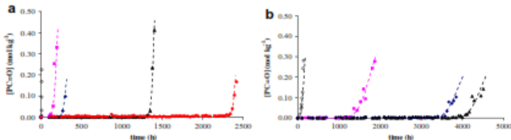
Fig. 1. Oxidation kinetics at 130 (a) et 100 °C (b) for pure PP (○), PP + 0.05% (■), PP + 0.1% (◆), PP + 0.2% (▲) and PP + 0.5% Irganox 1010 (●).
