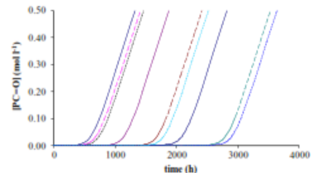
Fig. 4. Simulation of carbonyl build up curves at 80 °C using model M_1 with parameters given in Table 3. [POOH]_0 = 10^{-2} \text{ mol l}^{-1} (—), [POOH]_0 = 10^{-3} \text{ mol l}^{-1} (---), [POOH]_0 = 10^{-4} \text{ mol l}^{-1} (····), [POOH]_0 = 10^{-5} \text{ mol l}^{-1} (-·-·-).
