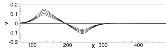
FIG. 1. Suction-and-blowing profiles imposed at the upper boundary for the v -component of the velocity.
