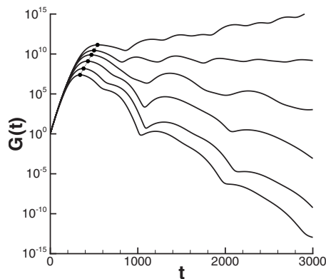
FIG. 25. Optimal energy gain curves obtained by the global eigenvalue analysis with N=400 modes for increasing Reynolds numbers: from the bottom curve to the top one, Re=190, 200, 207, 213, 219 , and 225 , respectively.
