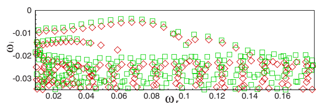
FIG. 38. (Color online) Global spectrum obtained for Re=200 with a (200 \times 40) grid (squares) and a (250 \times 48) grid (diamonds).
