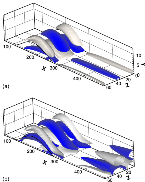
FIG. 5. (Color online) Isosurfaces of spanwise vorticity of the perturbation for the most amplified steady modes (a) M_S and (b) M_G at Re=200 . The black line is the separation streamline, whereas the dark and light surfaces represent the 0.15 and -0.15 values, respectively. The perturbations have been normalized by their maximum value.
