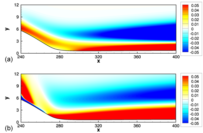
FIG. 12. (Color online) Spanwise vorticity of the perturbation for the global mode M_G (a) and for the solution obtained by the space integration of the Gortler equations (b), represented over the streamline \phi_G .
