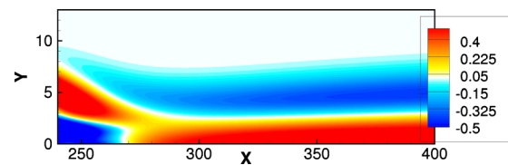
FIG. 22. (Color online) Blow-up of the shaded contours of the spanwise vorticity of the perturbation extracted from the DNS initialized by the optimal initial perturbation with amplitude A_0=10^{-6} at z=42 and t=2500 . The perturbation has been normalized by its maximum value.
