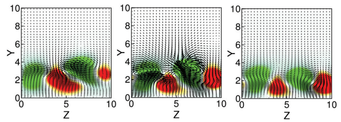
FIG. 6. (Color online) Contours of the streamwise components of the perturbation and cross-stream velocity vectors at x = 650 and t = 610, 640, 660 (from left to right) obtained using a DNS initialized by the linear optimal perturbation with E_0 = 0.075643438 (maximum value, w = 0.015 ). Shaded contours represent values from u = -0.06 (lighter contours, green online) to u = 0.04 (darker contours, red online) (enhanced online). [URL: http://dx.doi.org/10.1063/1.3589842.2 ]
