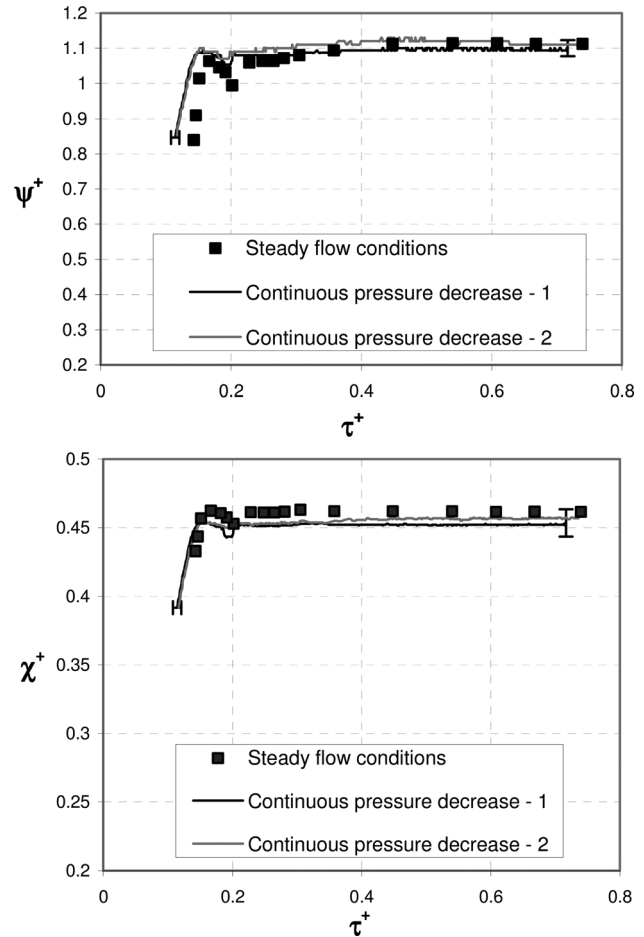
Fig. 5 (a) Head coefficient drop charts and (b) torque coefficient drop charts (IND3, N_{ref} , Q_n )
