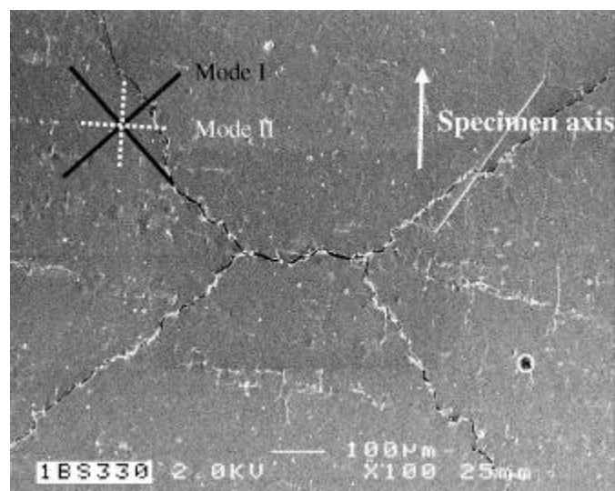
Fig. 20. SEM view of a replica done on the sample C36TO04 after 8 \times 10^5 cycles.
