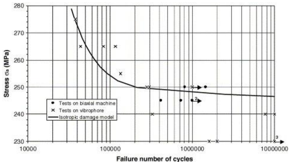
Fig. 22. Experimental data and predicted Wöhler curve in tension.
