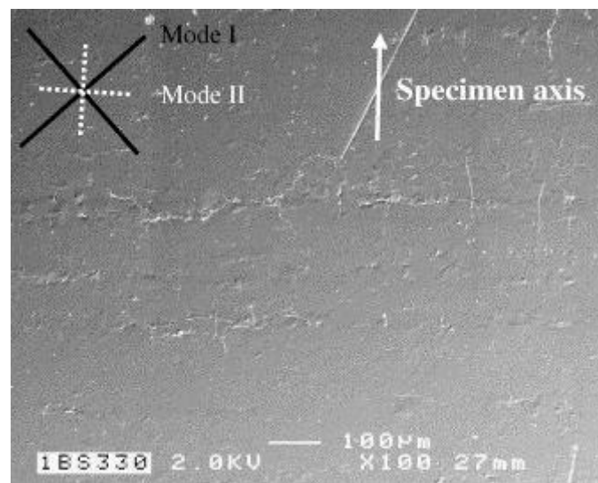
Fig. 17. SEM view of a replica done on the sample C36TO04 after 5 \times 10^5 cycles.
