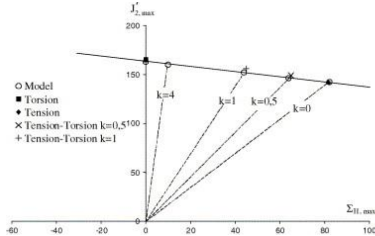
Fig. 23. Predicted threshold endurance curve (at 10^6 cycles and for a 50% failure probability) and experimental data in the plane usually used by Papadopoulos (J'_{2,max}, \Sigma_{H,max}) .
