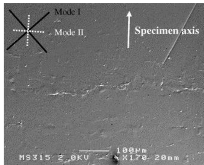
Fig. 16. SEM view of a replica done on the sample C36TO04 after 4 \times 10^5 cycles.
