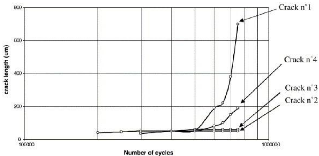
Fig. 6. Crack length in function of number of applied cycles for four cracks occurring on the specimen C36TR05 submitted to tension.
