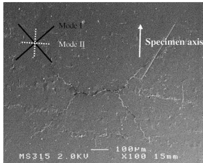
Fig. 19. SEM view of a replica done on the sample C36TO04 after 7 \times 10^5 cycles.
