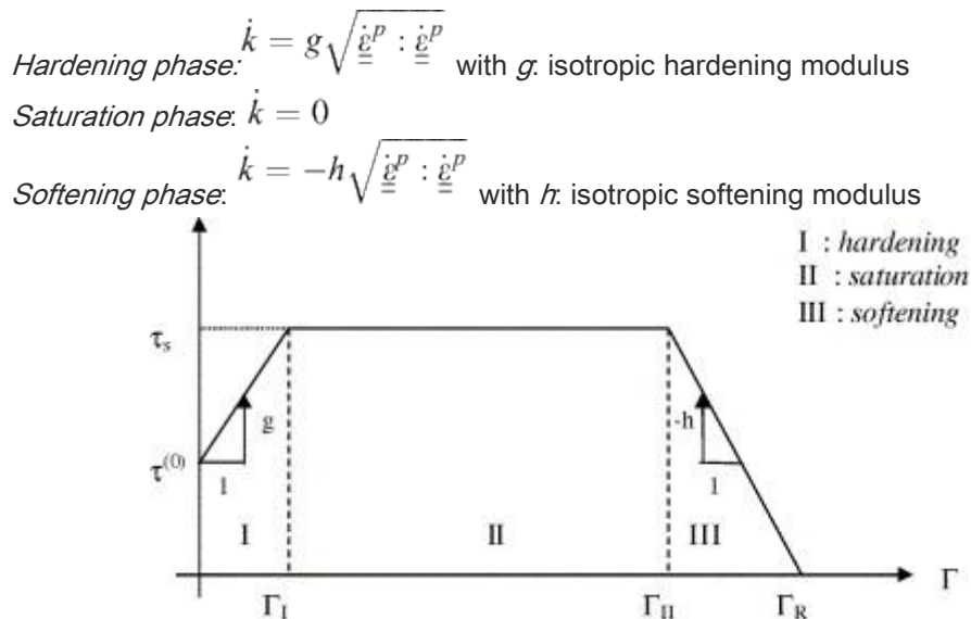
Fig. 2. Diagrammatic representation of the construction of the three plastic behavior proposal [1].
