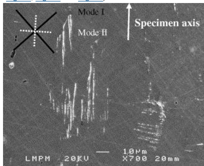
Fig. 12. SEM view of a sample loading in torsion, after only 10^5 cycles. The failure number of cycles of this sample is equal to 4 \times 10^5 cycles. This view gives good example of accumulative plastic strain on critical mode II plans.
