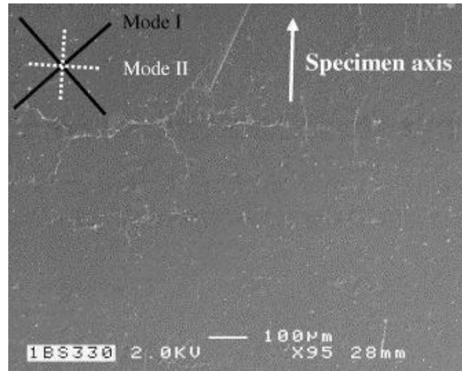
Fig. 18. SEM view of a replica done on the sample C36TO04 after 6 \times 10^5 cycles.
