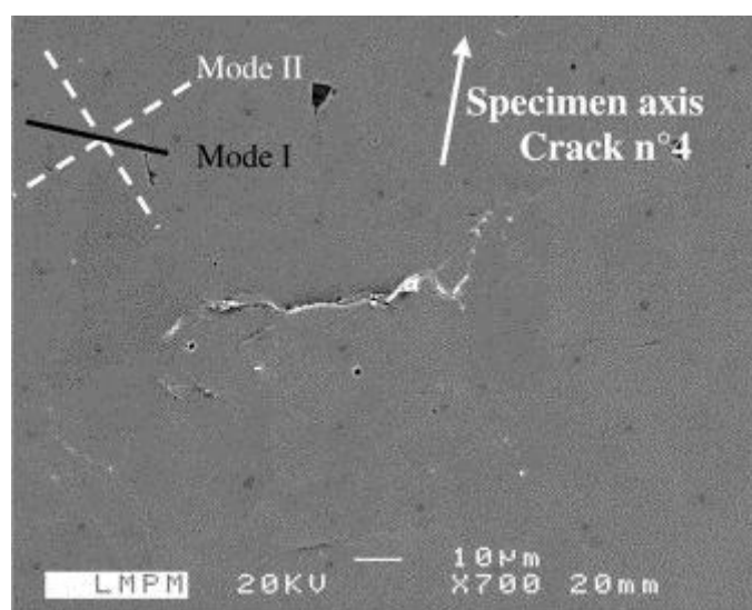
Fig. 9. SEM view of the crack No. 4 on the sample C36TR05 after 4 \times 10^5 cycles.
