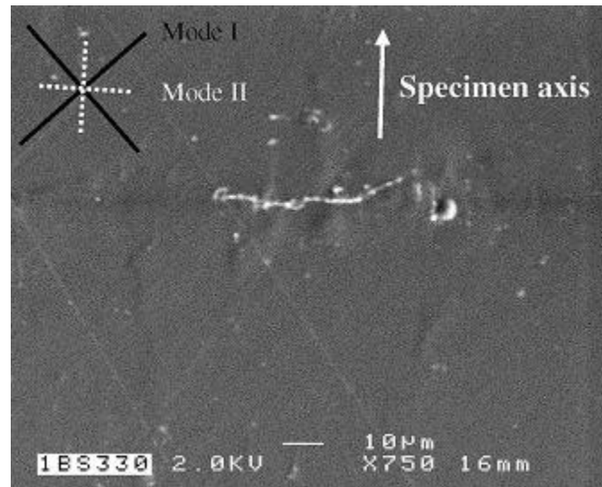
Fig. 13. SEM view of a replica done on the sample C36TO04 after 10^5 cycles.
