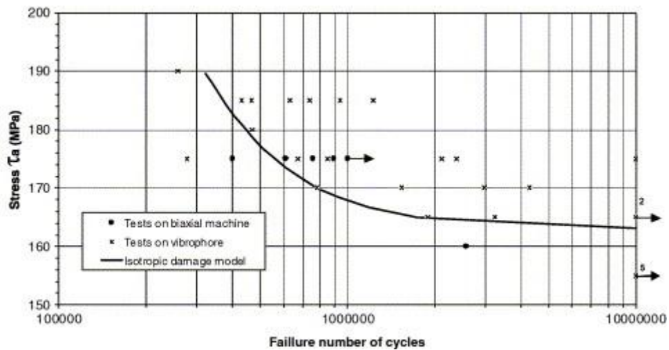
Fig. 21. Experimental data and predicted Wöhler curve in torsion.
