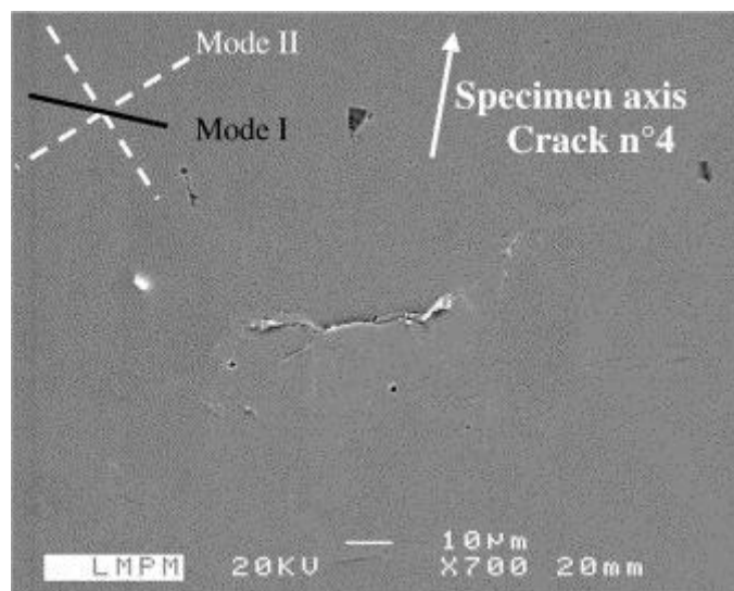
Fig. 8. SEM view of the crack No. 4 on the sample C36TR05 after 3 \times 10^5 cycles.
