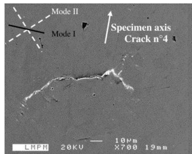
Fig. 10. SEM view of the crack No. 4 on the sample C36TR05 after 6 \times 10^5 cycles.
