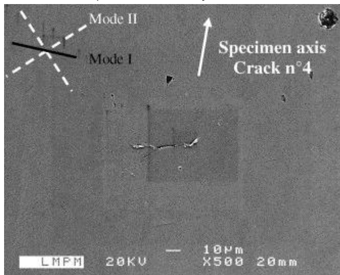
Fig. 7. SEM view of the crack No. 4 On the sample C36TR05 after 2 \times 10^5 cycles.
