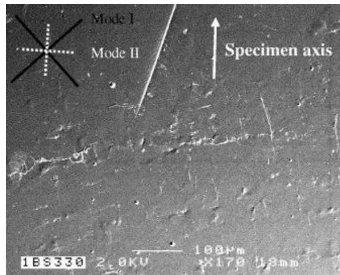
Fig. 15. SEM view of a replica done on the sample C36TO04 after 3 \times 10^5 cycles.
