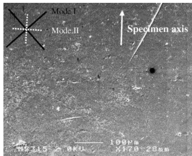
Fig. 14. SEM view of a replica done on the sample C36TO04 after 2 \times 10^5 cycles.
