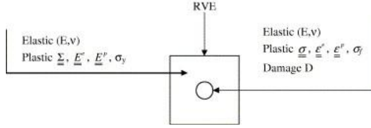
Fig. 1. Diagrammatic representation of the construction of the two's scale model [5].
