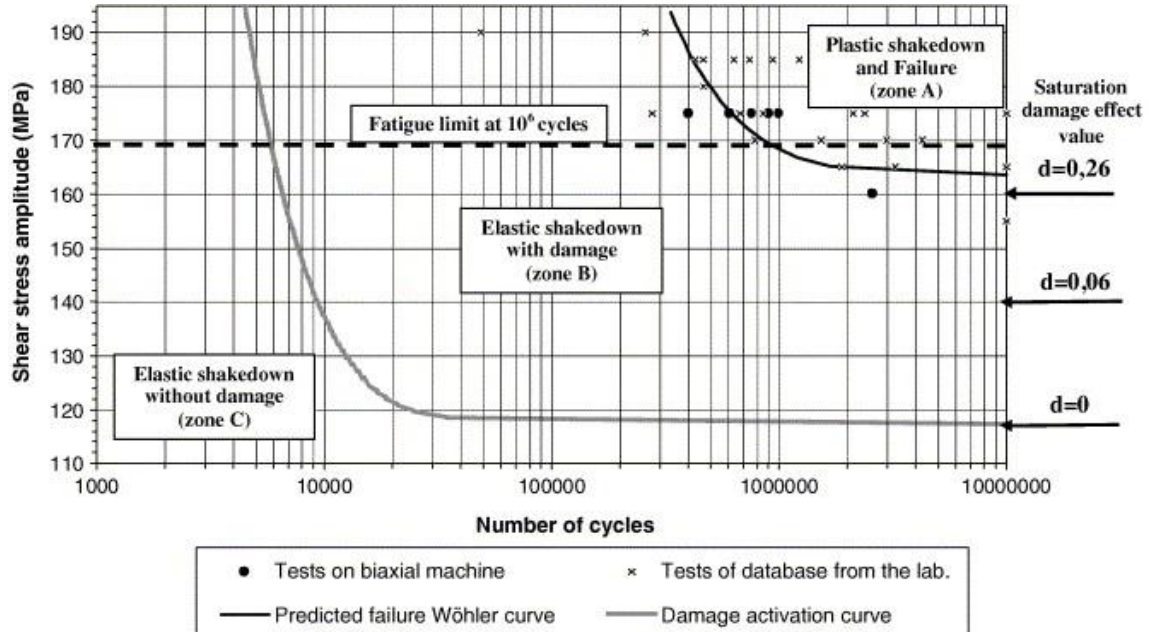
Fig. 25. Predicted failure curve, damage activation curve, and experimental data in a Wöhler diagram for pure alternative torsion loading.
