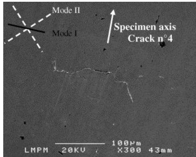
Fig. 11. SEM view of the crack No. 4 on the sample C36TR05 after 7,5 \times 10^5 cycles.
