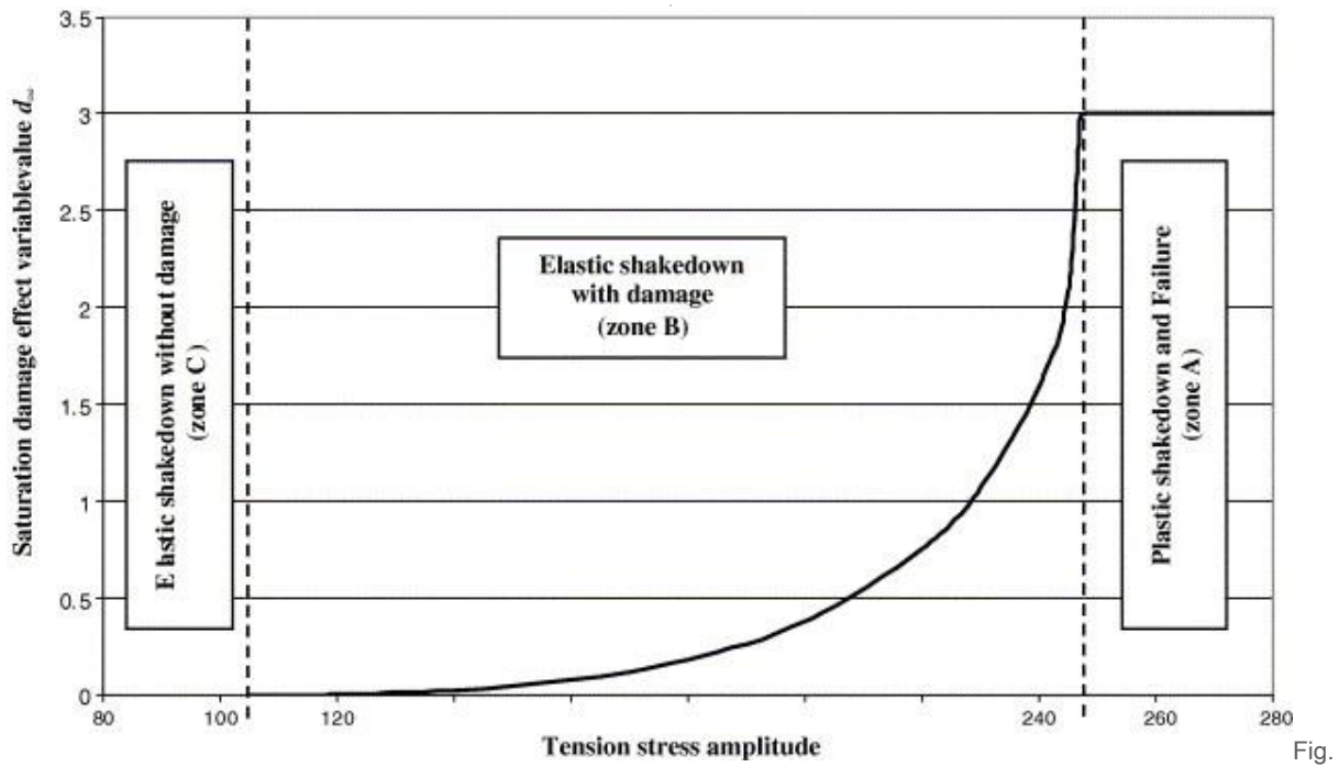
Fig. 27. Saturation damage effect variable d_s according to constant stress amplitude of the tension loading.
