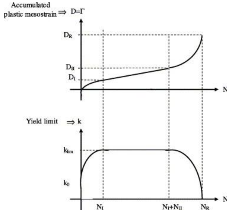
Fig. 3. Damage in terms of accumulated plastic mesostrain and yield limit evolutions in the three phases of behaviour [2].
