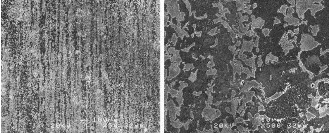
Figs. 4 and 5. SEM views of the microstructure of the ferrito-pearlitic C36 steel.
