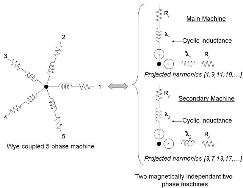
Figure 1: Multimachine decomposition for a wye-coupled 5-phase machine
