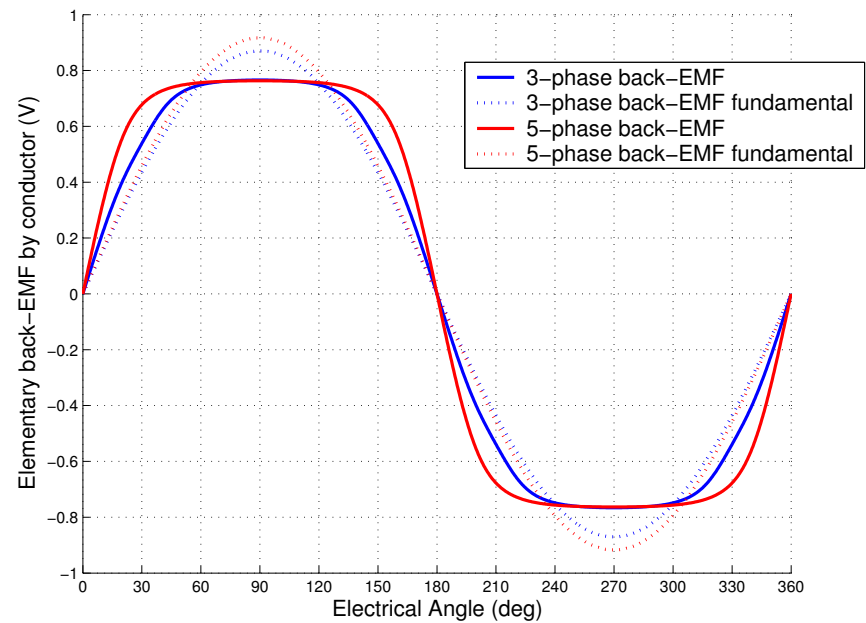
Figure 4: Comparison of the elementary back-EMF by conductor \epsilon_{cd}(3) and \epsilon_{cd}(5) (analytical estimations)
