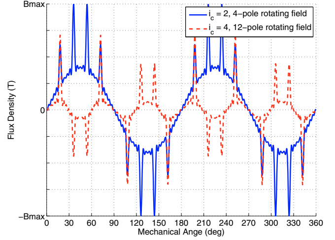
Fig. 5. (Color online) Comparison of the air gap flux density obtained with i_c = 2 and i_c = 4 for a 5-phase machine (winding of Fig. 2 where (p, N_s) = (2, 20) ).
