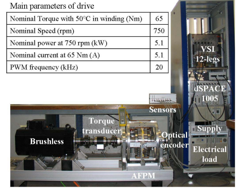
Fig. 3. Experimental setup
