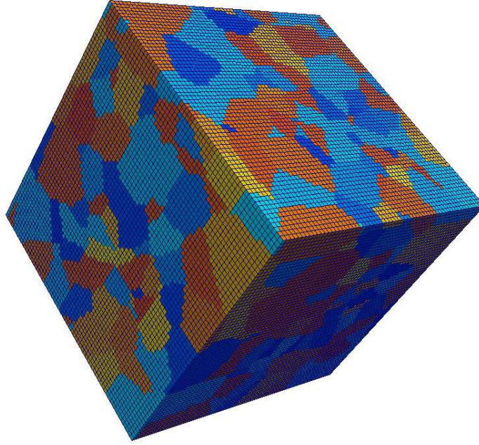
Fig. 8. Representation of the discretized microstructure of the C35 steel grade. Pearlitic voxels appear with a red/orange color while ferritic voxels appear with a blue color.
