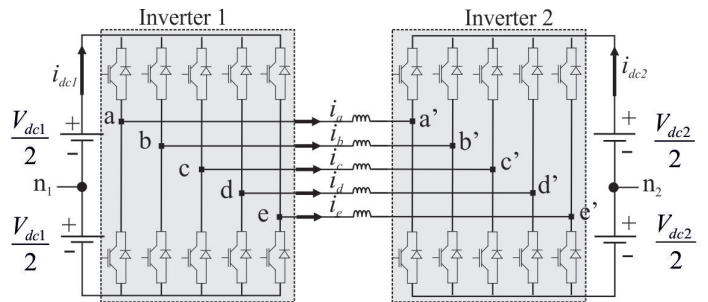
Figure 3. Double-ended inverters open-winding five-phase PM machine structure
