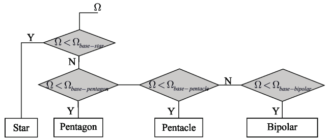
Figure 5. Flow-chart control strategy
