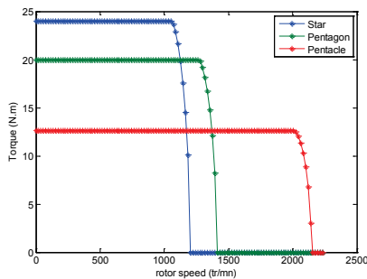
Figure 2. Torque-speed characteristics with different stator configurations given in Figure 1
