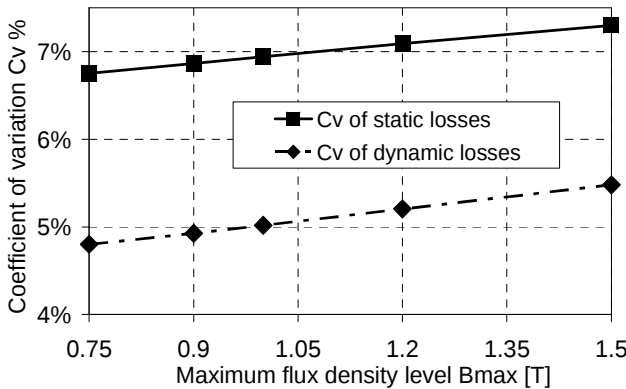
Fig 6: Coefficient of Variation of static and dynamic components of losses for SS group at 50Hz
